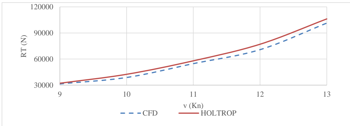
Fig. 6. Comparison of CFD Ship Resistance with Holtrop
