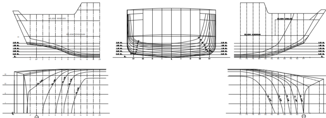
Fig. 1. Lines Plan of KMP. Bontoharu 1050 GT
