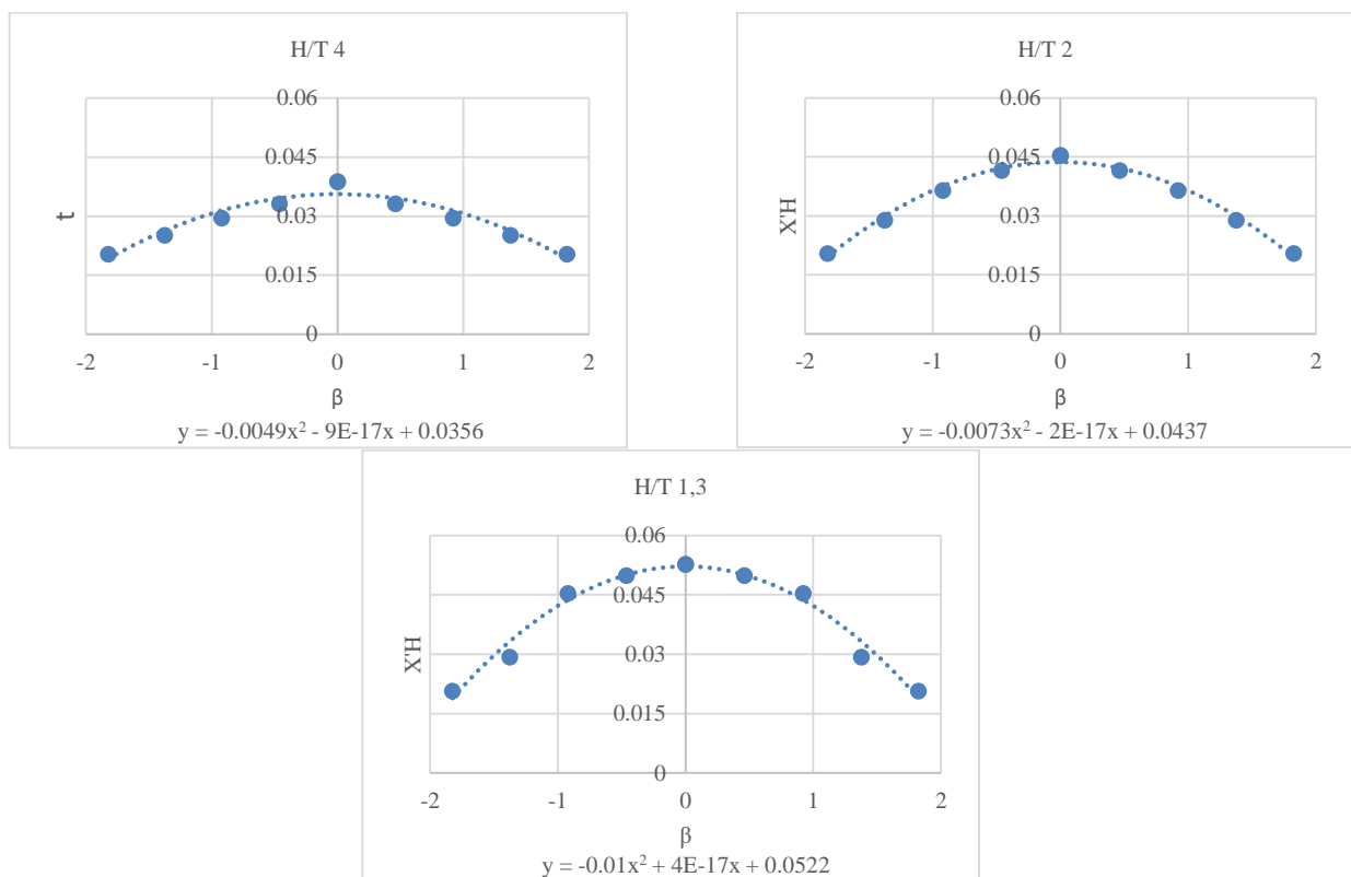
Fig. 8. Graph of X'H Simulation Results, with Variations in Depth
