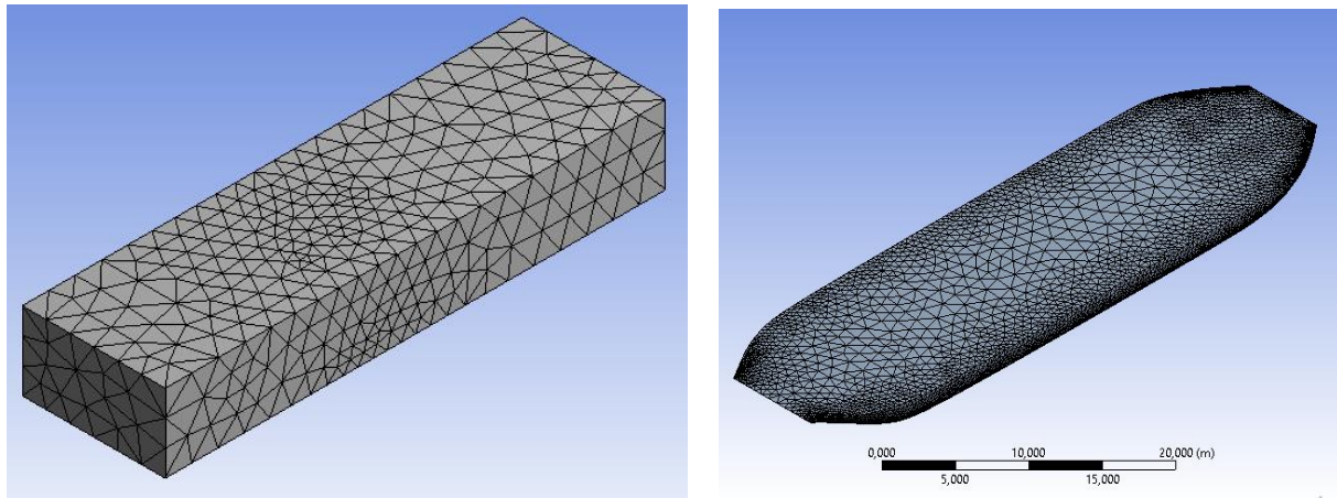
(a) (b) Fig. 4. (a) Hull Meshing (b) Meshing with Fluid Domain
