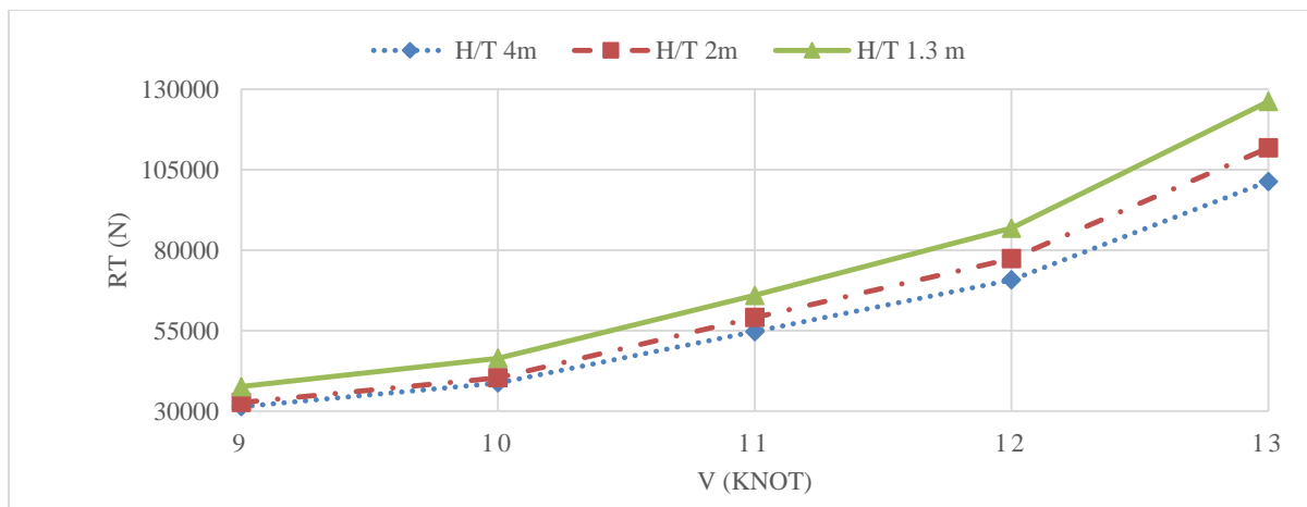
Fig. 7. KMP Bontoharu Ship Resistance with Depth Variation
