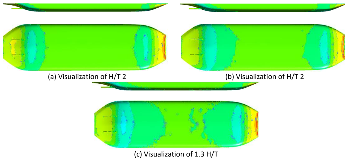
Fig. 9. Pressure Characteristics from CFD Simulation
